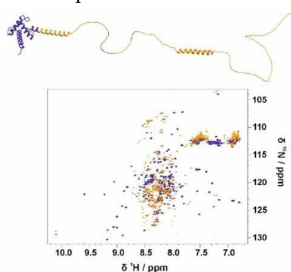
Fig. 1. Structural model of TAZ4 is reported on top of the figure. Relaxation-edited 1 H- 15 N HSQC spectrum is reported on the bottom part of the figure.
