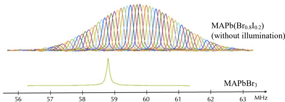
Fig. 1. 81 Br NQR spectra of MAPbBr 3 and MAPb(Br 0.8 I 0.2 ) 3
