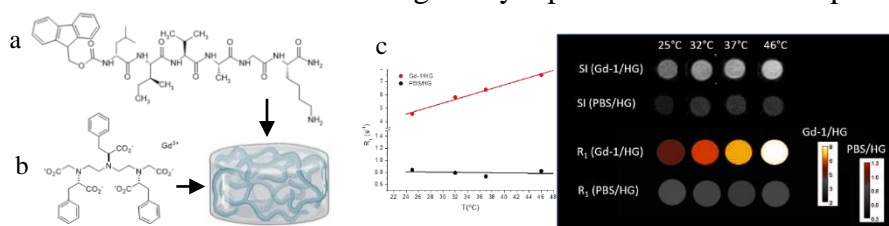
Fig.1 a) structure of peptide Fmoc-K2; b) structure of Gd-1; c) T_{1w} images and T_1 maps at 1T.
