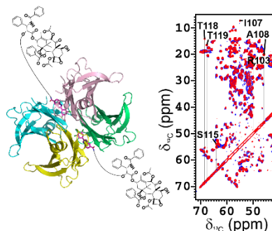
Fig. 1. Solid-state NMR analysis of protein-drug conjugate
