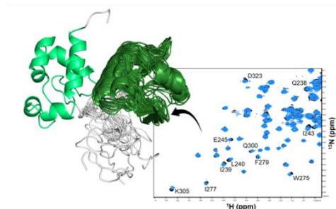
Fig. 1. NMR spectra and structure of LaRP4B.
