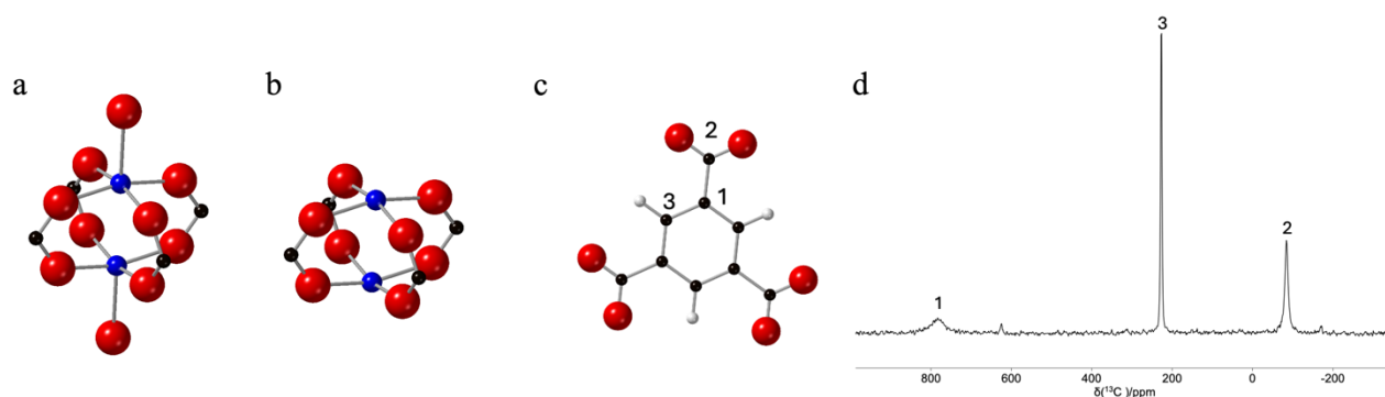
Fig. 1. Cu(II) paddlewheel dimers SBUs of HKUST-1 in the (a) hydrated form with water molecules occupying the axial position and in the (b) evacuated form. (c) The structure of the btc linker. (d) 13 C spectrum of evacuated HKUST-1.
