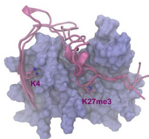
Figure 1: Model of PHDV5HCH NSD2 :H3K4K27me3 complex. Superposition of three representative binding poses extracted from three independent MD calculations
