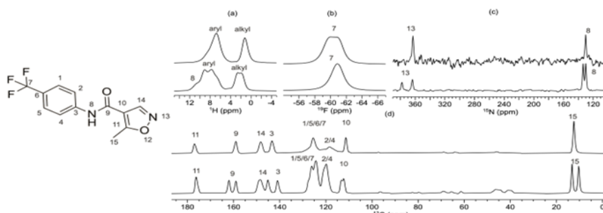
Fig. 1. 1 H (a), 19 F (b), 15 N (c) and 13 C (d) MAS spectra of the two different polymorphs of Leflunomide, \langle \square \rangle and \langle \otimes \rangle , with signal assignment.
